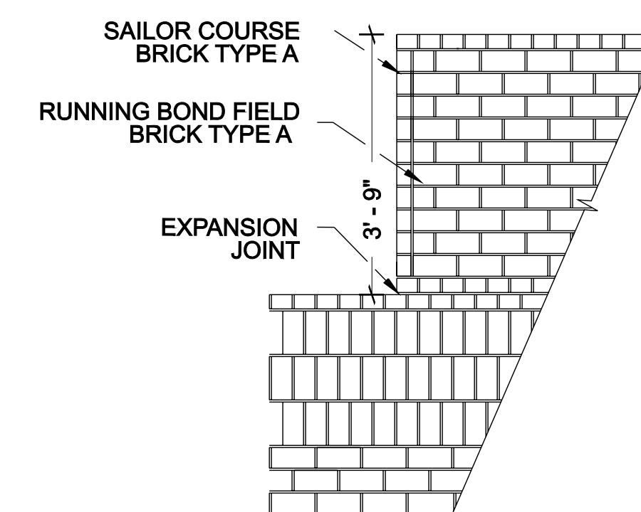
E L-3 BENCH BUMP OUT PAVING TYPE 2 1/2" = 1' - 0"
