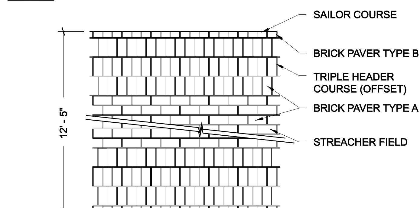
B L-3 12'-5" WALKWAY PAVING PATTERN 1/2" = 1' - 0"
