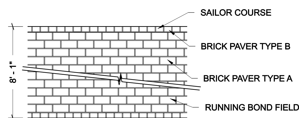
C L-3 8'-1" WALKWAY PAVING PATTERN 1/2" = 1' - 0"
