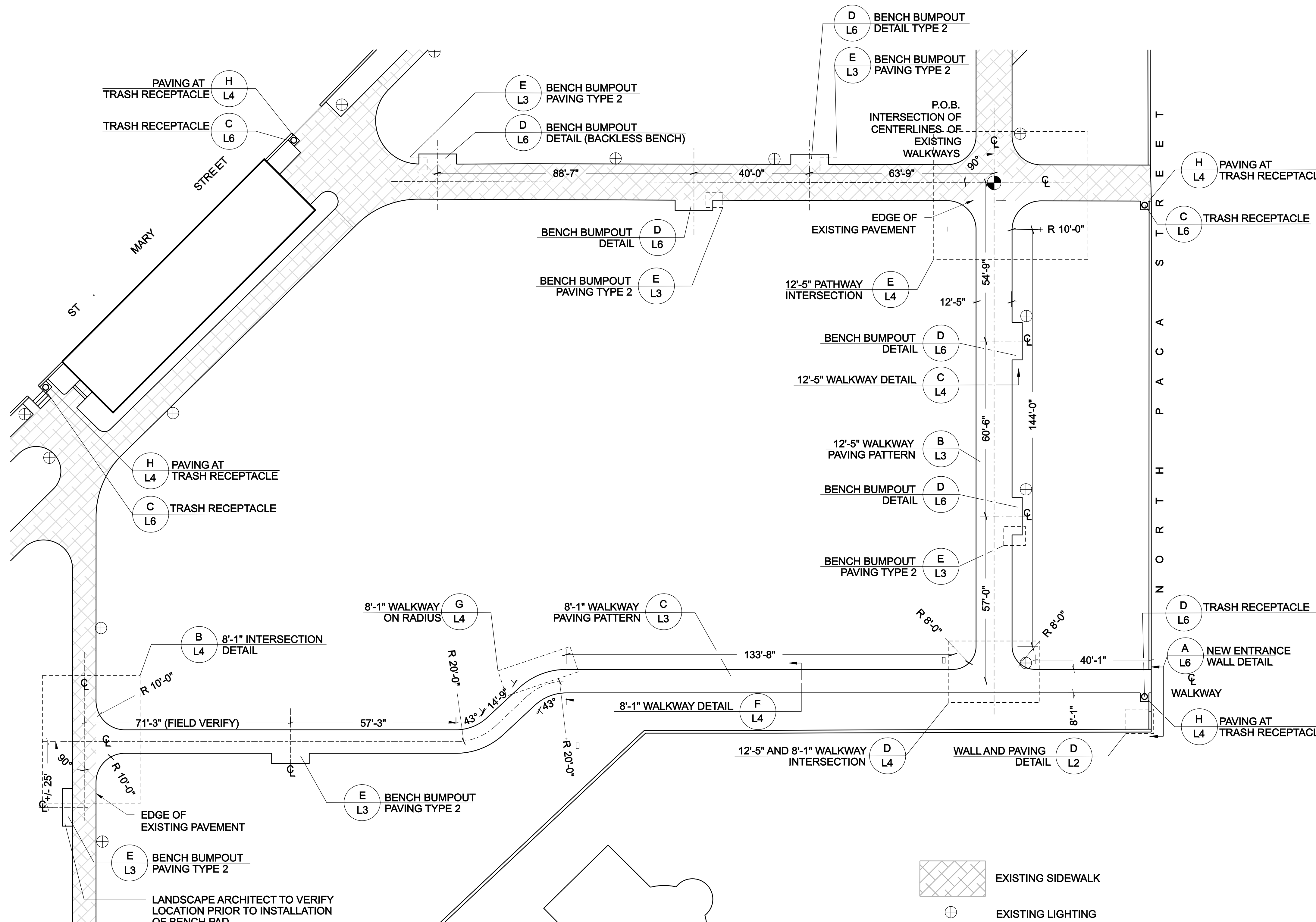
A L-3 NEW PATHWAY LAYOUT PLAN 1" = 20' - 0"
